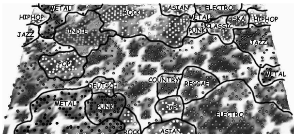
Figure 5: U-Map of the tagged music data.
